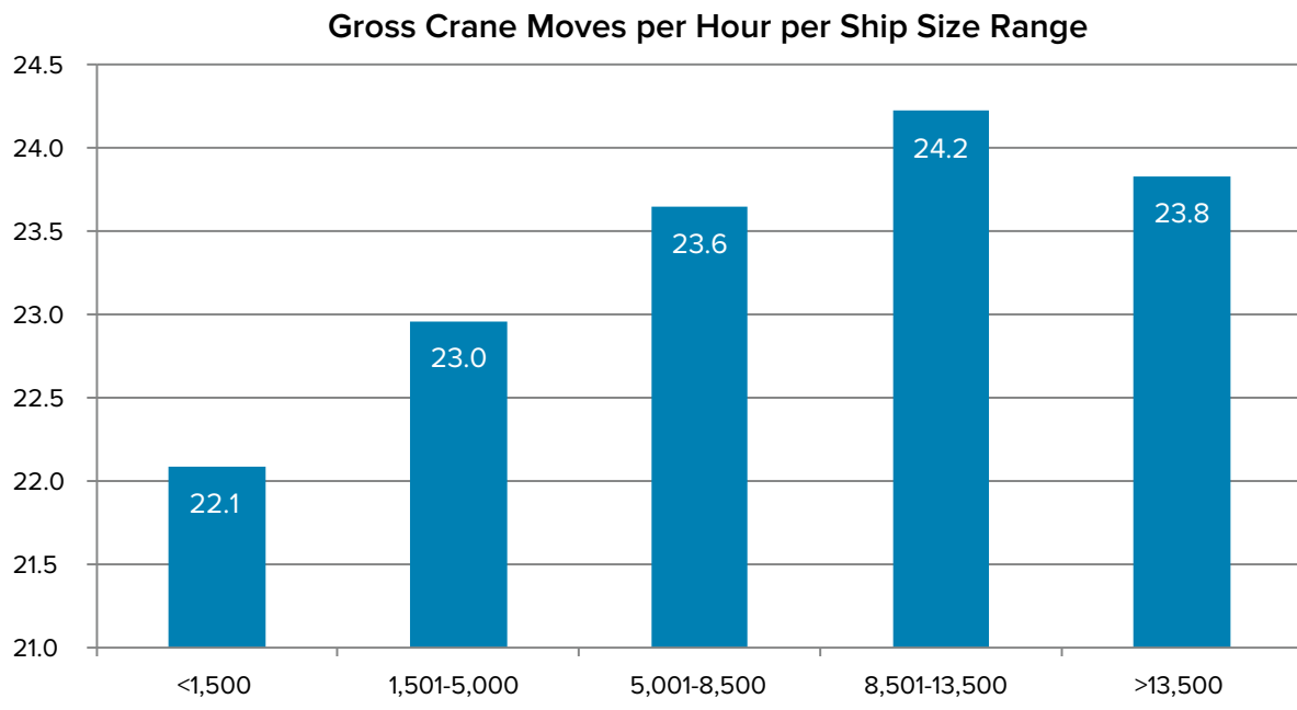
FIGURE 2.7 • Gross Crane Productivity
