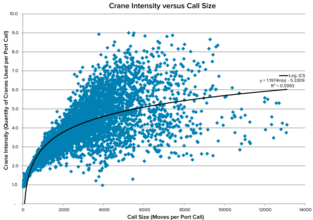
FIGURE 2.5. • Regression Analysis: Crane Intensity versus Call Size
