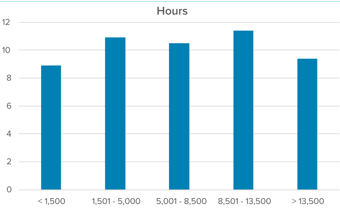
FIGURE 2.2. • Average Arrival Times at Hub Ports per Ship Size Range
