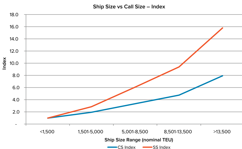
FIGURE 2.6. • Relationship between Global Ship Size and Call Size
