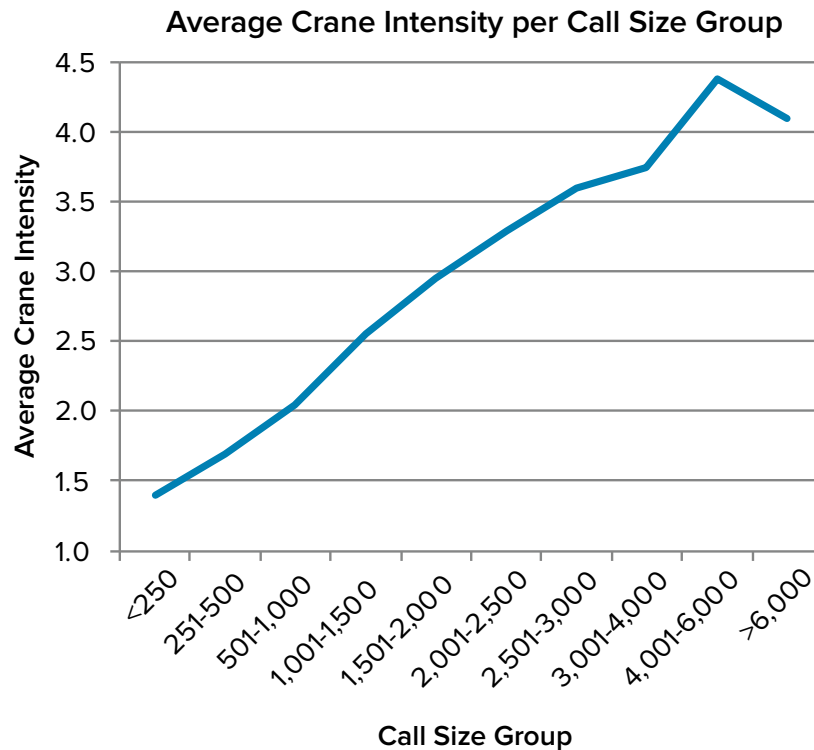
FIGURE 2.8. • Average Crane Intensity per Defined Call Size Group
