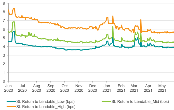
SL Returns to Lendable : Jun 20 to May 21
